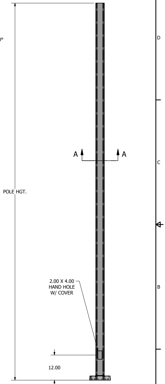
POLE DETAIL
